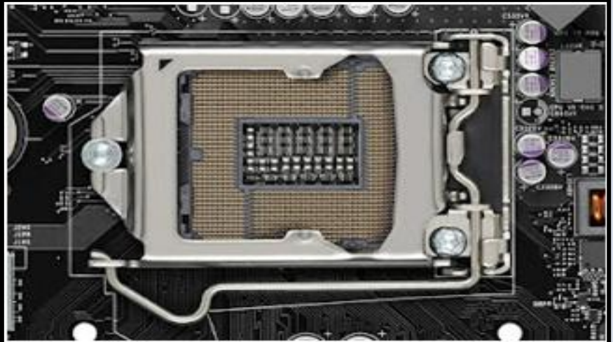
Socket LGA 1156 Core i3 و Core i5 و Core i7
