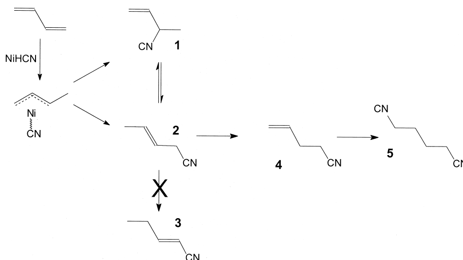
FIGURE 70 Hydrocyanation of butadiene leading to adiponitrile.
