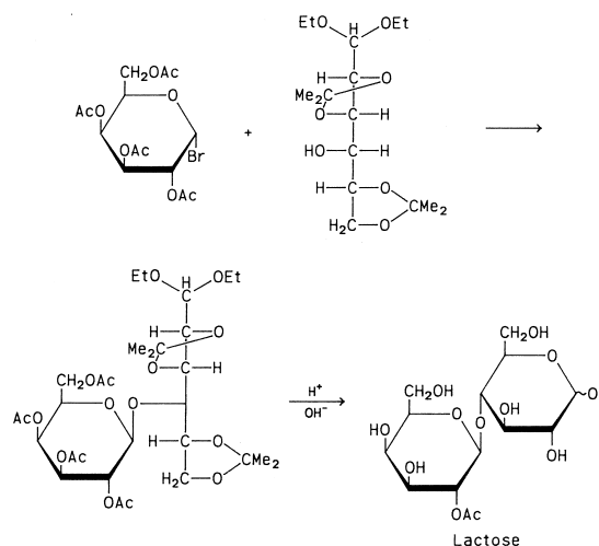
SCHEME 23 Synthesis of lactose.
