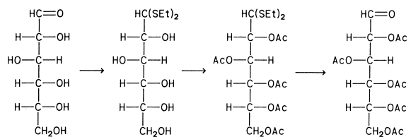
SCHEME 9 Formation of acyclic aldoses from dithioacetals.
