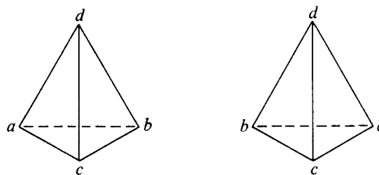
FIGURE 1 Tetrahedral molecule Cabcd (the carbon atom at the center of the tetrahedron is conventionally not shown). [Reprinted with permission from Eliel, E. L., and Wilen, S. H. (1994). “Stereochemistry of Organic Compounds,” Wiley, New York.]
