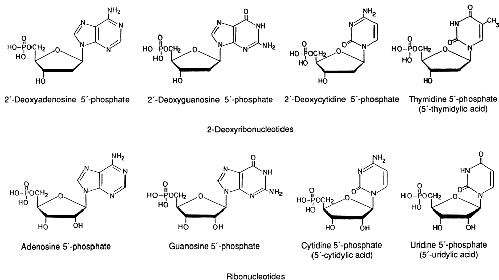
FIGURE 20 The four 2-deoxyribonucleotides found in DNA and the four ribonucleotides found in RNA.
