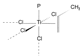
FIGURE 48 Cossee-Arleman site.
