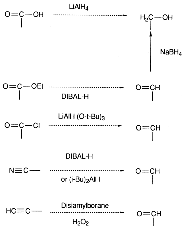
SCHEME 19 Action of reducing agents.
