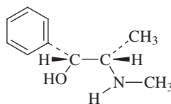
(-)-Ephedrine
