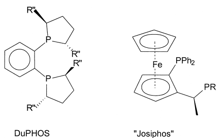
FIGURE 30 Chiral diphosphine ligands.
