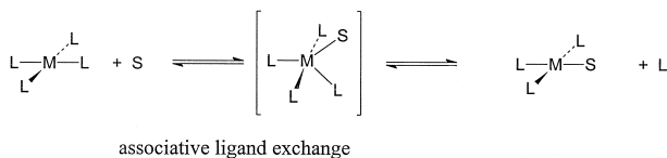
FIGURE 4 Dissociative and associative processes for ligand exchange.
