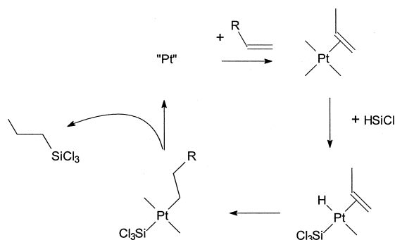
FIGURE 78 The Chalk-Harrod mechanism for hydrosilylation.
