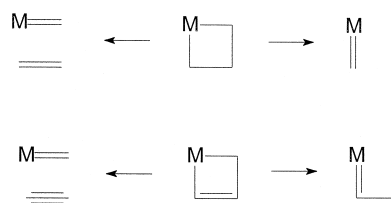
FIGURE 16 Retrocyclo metallation reactions.
