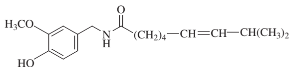
Capsaicine
