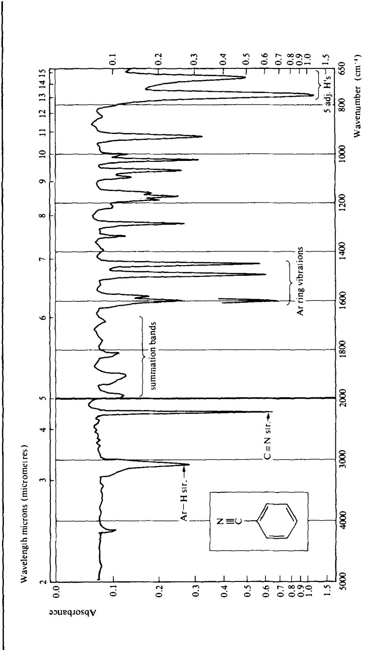
Fig. 3.39 Infrared spectrum of benzonitrile recorded as a liquid film.
