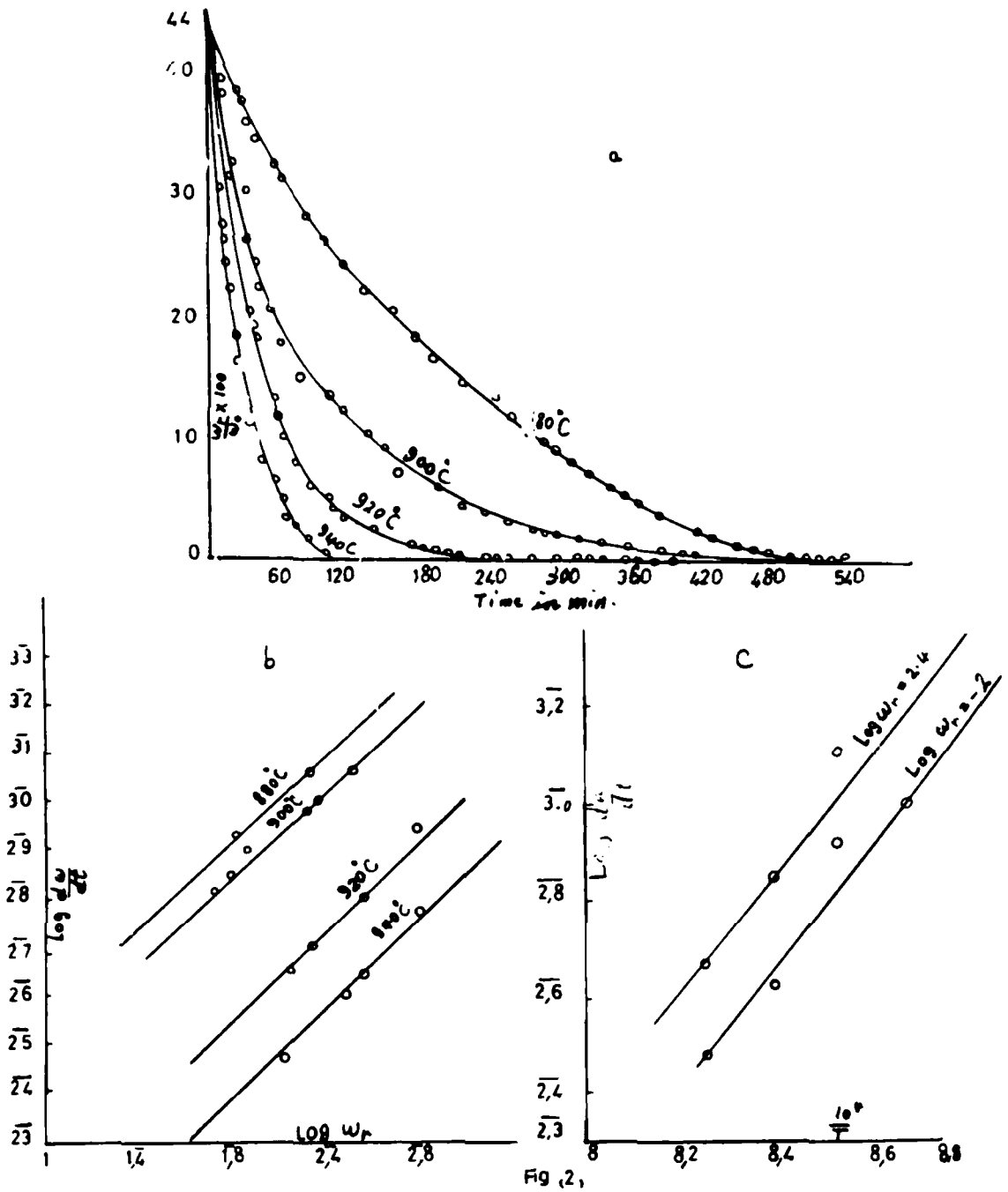
Fig.(2) Treatment (a) shows the relation between \frac{w}{w_0} \times 100 and time (t). treatment (b) shows the relation between \log \frac{dw}{dt} and \log w_r at constant temperatures 880°, 900°, 920° and 940°C. treatment (c) shows the relation between \log \frac{dw}{dt} and \frac{10^4}{T} for various values of \log w_r .
