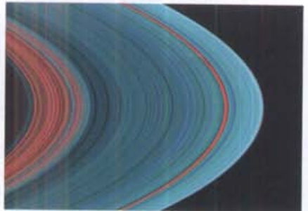
Saturn's Rings
