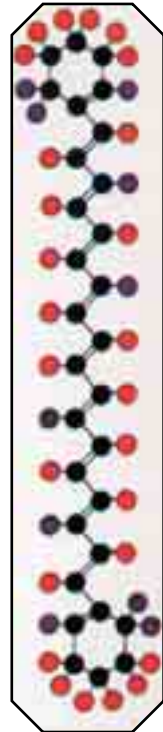
Molecular structure of the pigment beta carotene.
