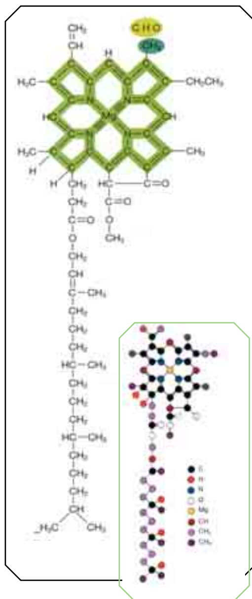
Chlorophyll, one of the vital elements in photosynthesis, consists of various atoms laid out according to the above formula.
