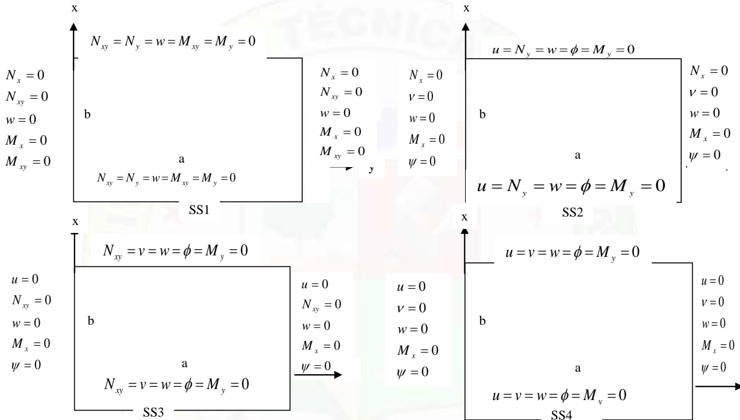
Fig. (1) Simply supported boundary conditions
